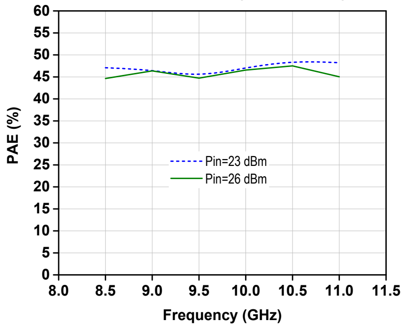
Power Added Efficiency vs Frequency
